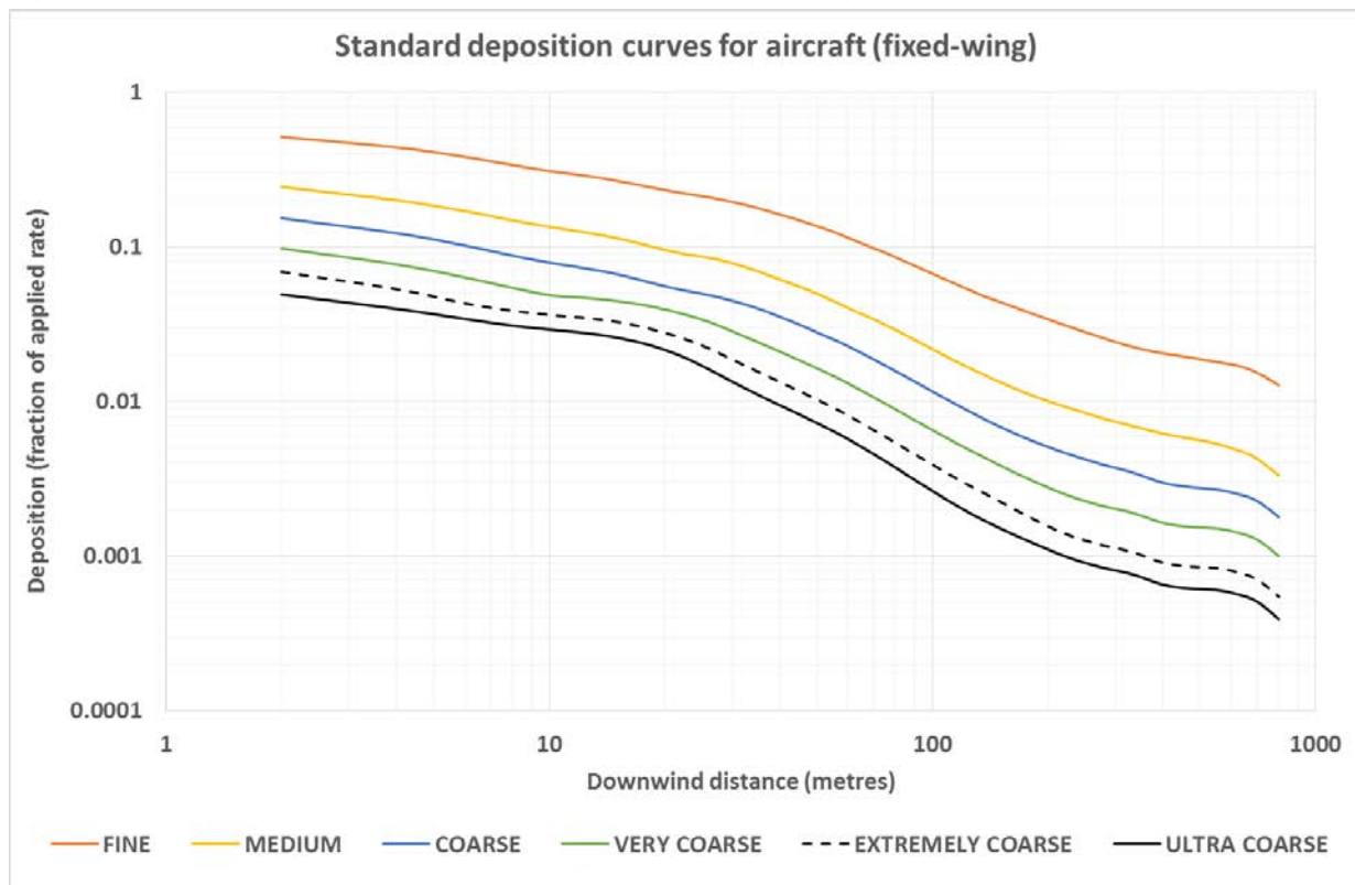
Figure 8: Chart of standard deposition curves for aircraft (fixed-wing)
