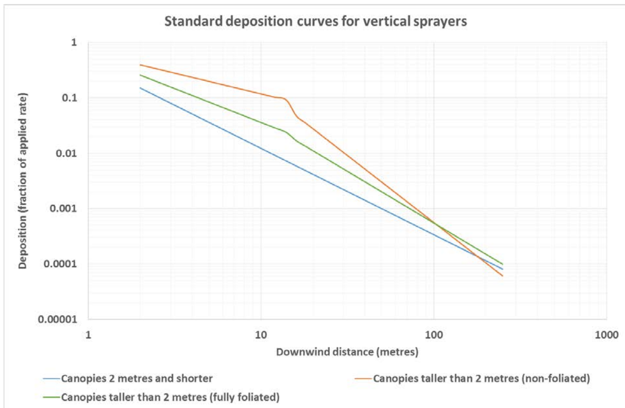
Figure 7: Chart of standard deposition curves for vertical sprayers
