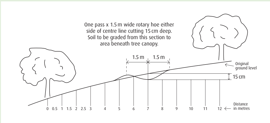
Cross section view: Where side slopes are greater than 10% an extra 2 metres in row spacing should be used in rows with drains. Drawing adapted from 'Soil Management in Orchards', NSW DPI Agnote DPI-331.
