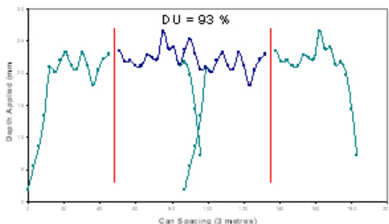
Figure 2: 270° gun rotation
